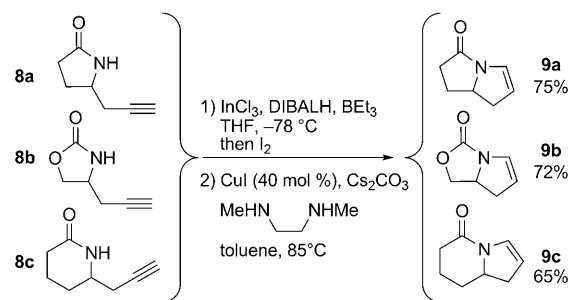
Scheme 2. Cyclization to form bicyclic heterocycles. The scheme shows individual reactions under the same conditions (i.e. 8a → 9a , 8b → 9b , 8c → 9c ). DIBALH = diisobutylaluminum hydride, THF = tetrahydrofuran.
