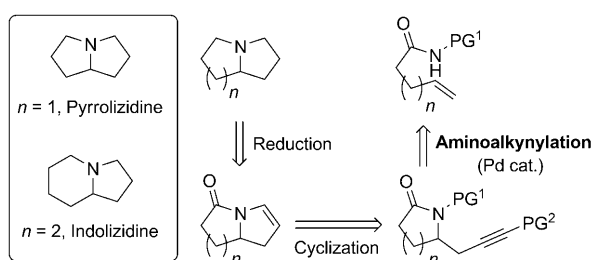
Scheme 1. Strategy for the synthesis of pyrrolizidines and indolizidines. PG = protecting group.
