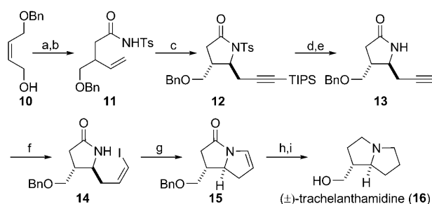
Scheme 3. Total synthesis of (±)-trachelanthamidine ( 16 ). Reaction conditions: a) CH 3 C(OEt) 3 , EtCO 2 H, 100 °C to 160 °C; then KOH, MeOH, reflux, 80 %; b) p -TsNCO, Et 3 N, THF, RT, 80 %; c) 5 mol % of PdCl 2 , LiCl, TIPS-EBX ( 2a ), EtOH, RT, 72 %; 83:17 d.r.; d) Li/naphthalene, THF, –78 °C, 77 %; e) TBAF, THF, 0 °C to RT, 98 %; f) 1) InCl 3 , DIBALH, 2) Et 3 B, 3) I 2 , THF, –50 °C, 95 %; g) 40 mol % CuI, Cs 2 CO 3 , N,N' -dimethylethylenediamine, toluene, 85 °C, 73 %; h) H 2 , Pd/C, MeOH, RT, quantitative; i) LiAlH 4 , THF, reflux, 94 %. TBAF = tetra- n -butylammonium fluoride.
